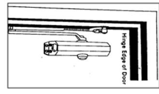
PARALLEL ARM INSTALLATION CLOSER IS INSTALLED ON PUSH SIDE OF DOOR
