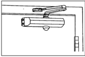
REGULAR ARM INSTALLATION CLOSER IS INSTALLED ON PULL/HINGE SIDE OF DOOR
