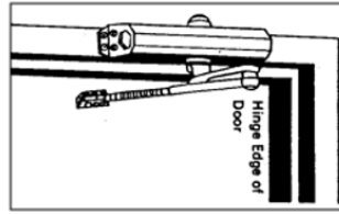
TOP JAMB INSTALLATION CLOSER IS INSTALLED ON FRAME ON PUSH SIDE OF DOOR
