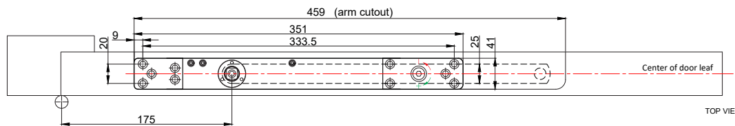
TOP VIEW
