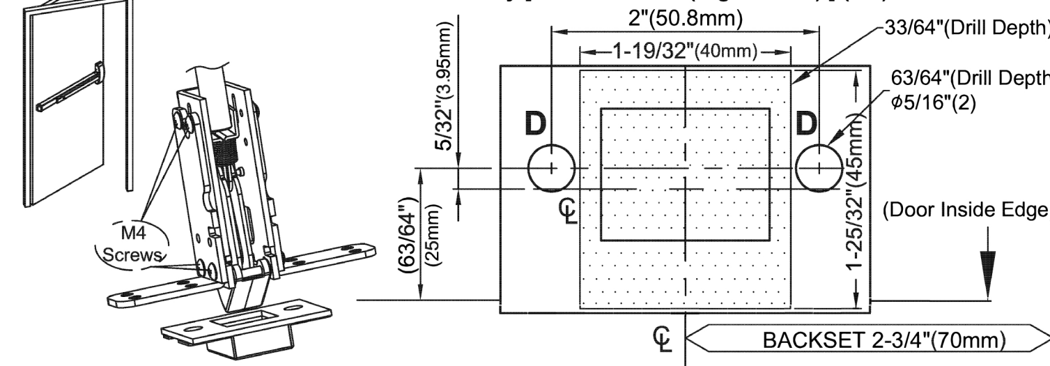
TEMPLATE of Bottom Latch Ass'y [ Bottom Strike (regular use) ] (1:1)
