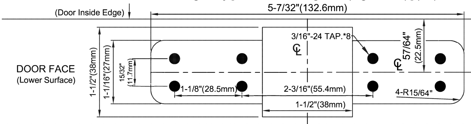
TEMPLATE of Bottom Latch Ass'y [ Bottom Strike (regular use) ] (1:1)
