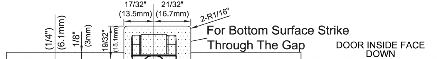
TEMPLATE of Bottom Latch Housing Ass'y [ Bottom Mounting Plate ] (1:1)
