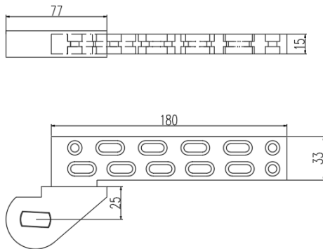
D7432/D6666-400 DOUBLE ACTION TOP CENTER AND BOTTOM STRAP
