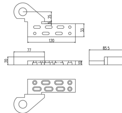
D44787-450 DINR OR DINL SINGLE ACTION UPPER TOP CENTER, SHOWING DINL
