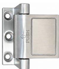
CDC44 SN
